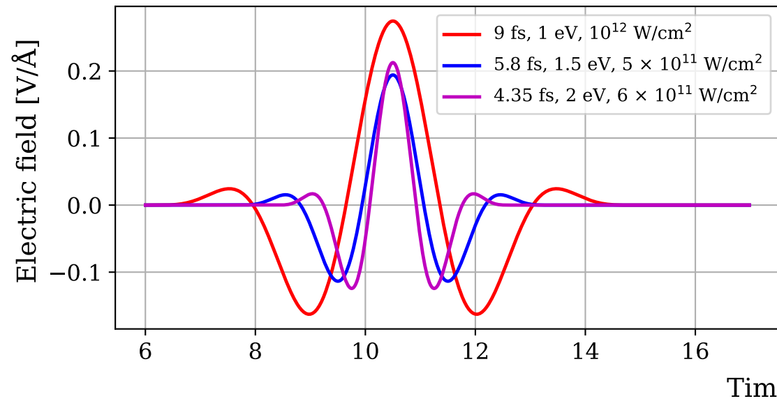
Pump electric field along the z-axis
