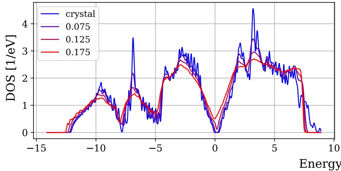
Displacement disorder
