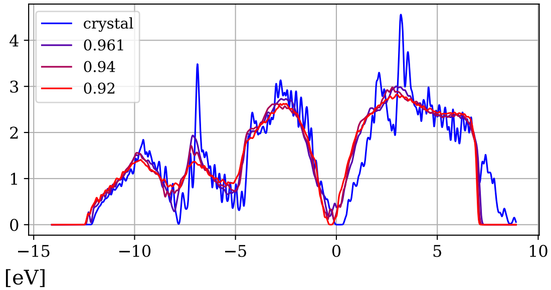
Amorphous disorder
