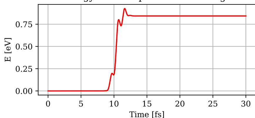
Energy transfer per unit cell along x
