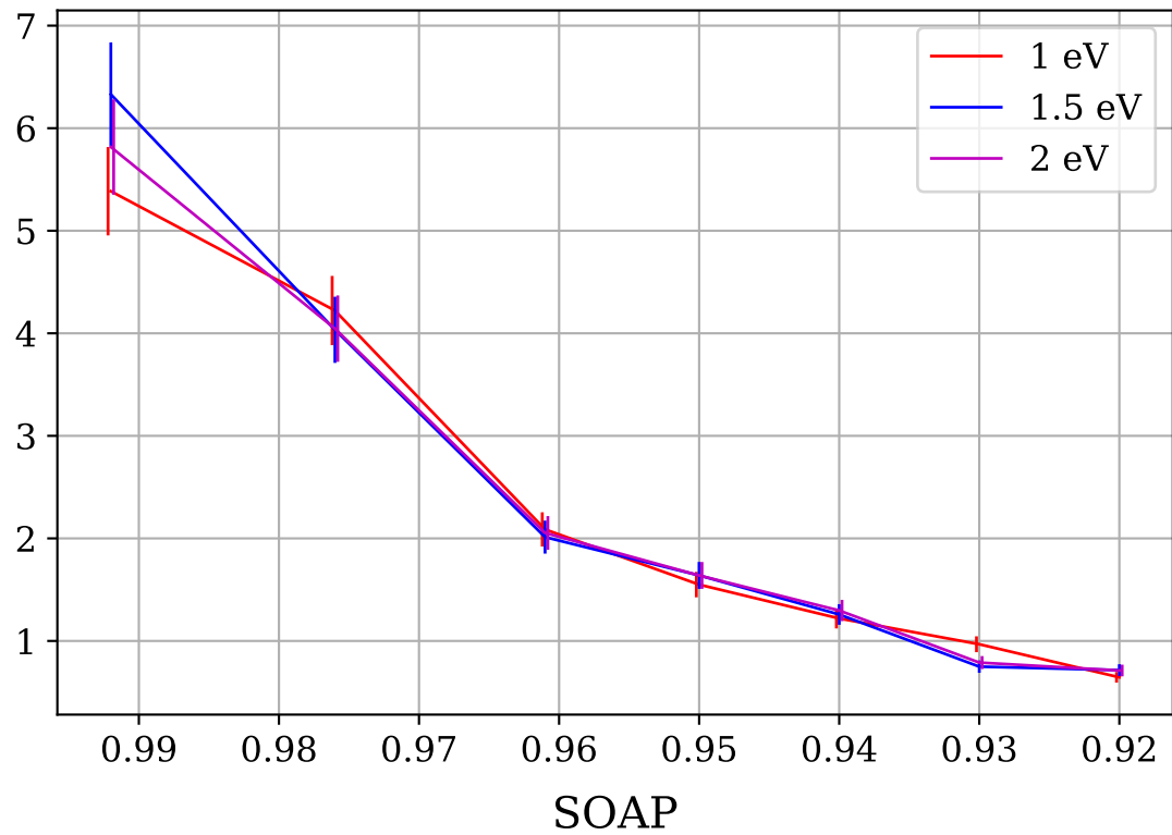
Amorphous disorder
