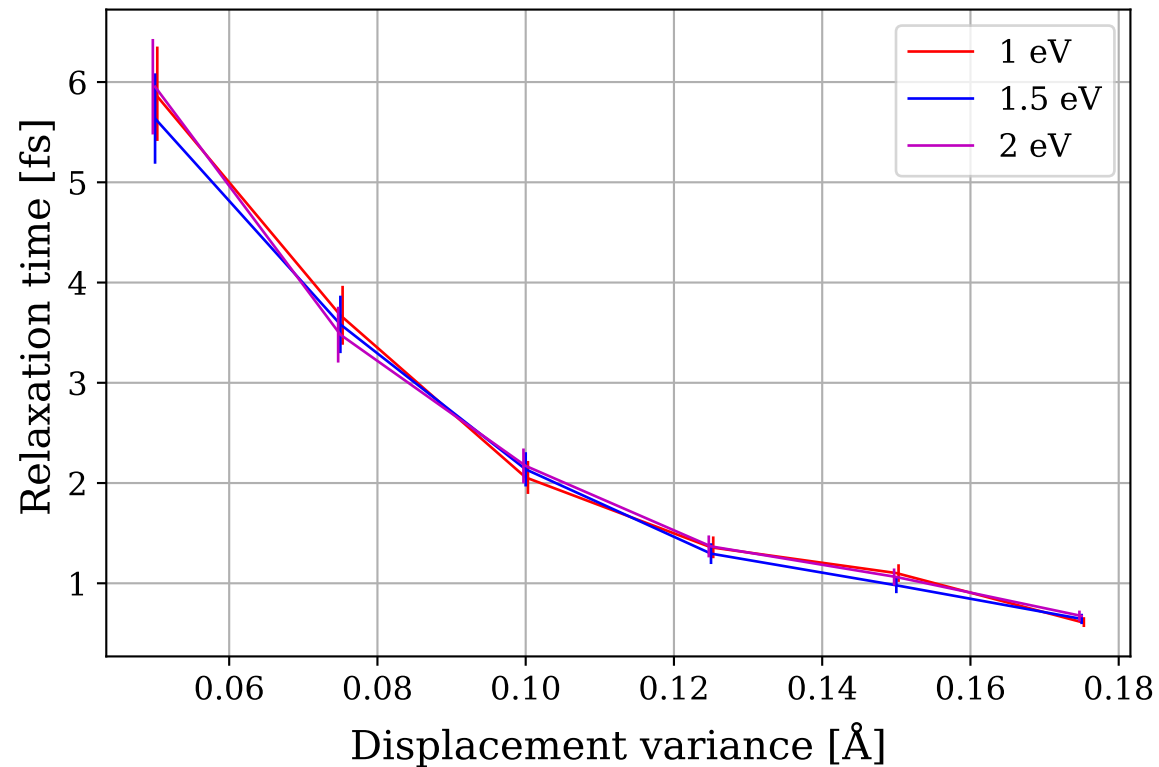
Displacement disorder
