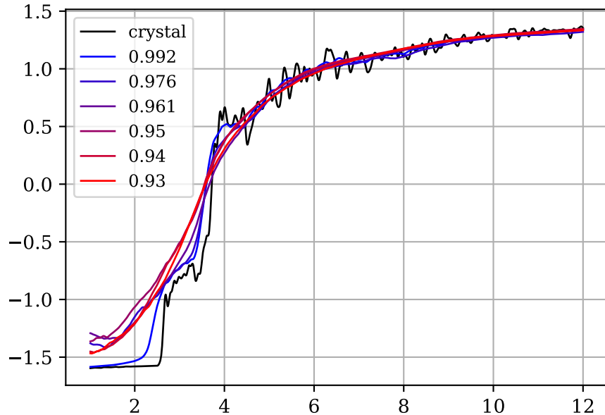
Amorphous disorder
