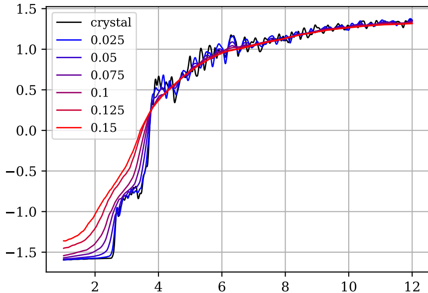
Displacement disorder
