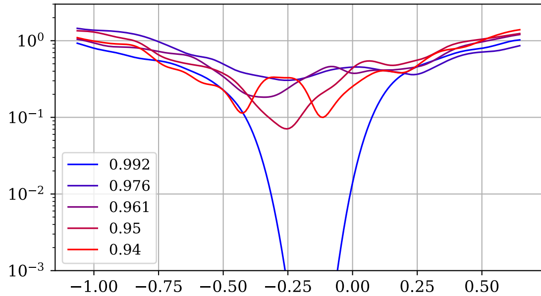
Amorphous disorder
