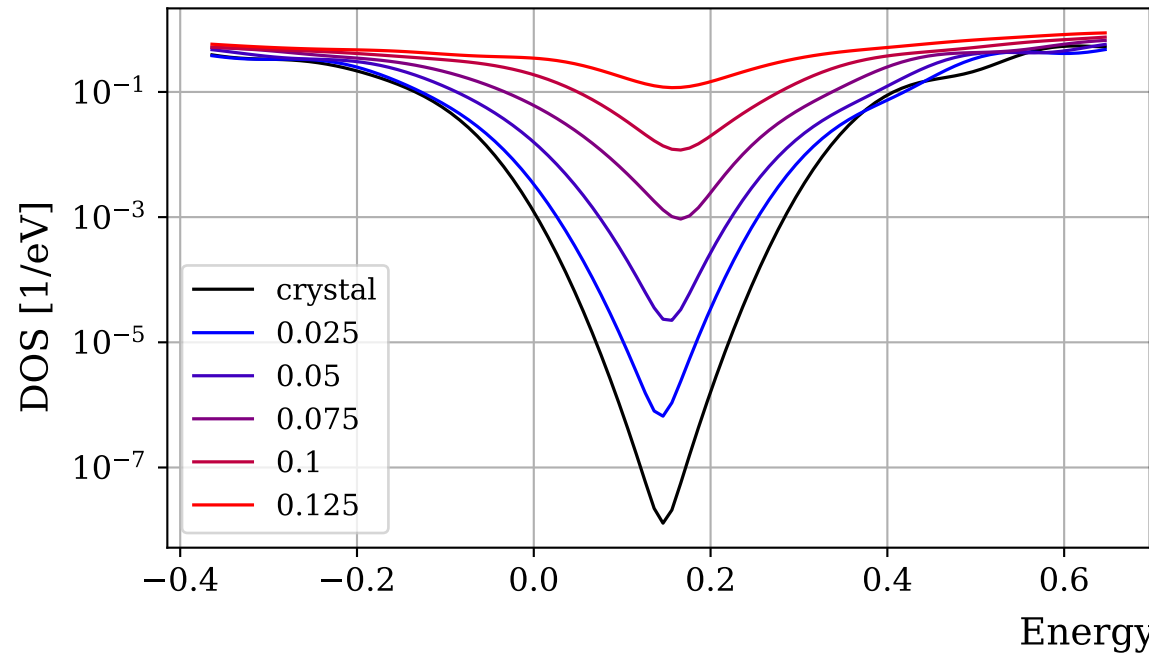
Displacement disorder
