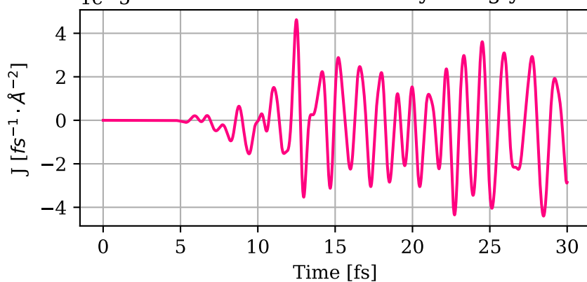
1e-5 \Delta matter current density along y
