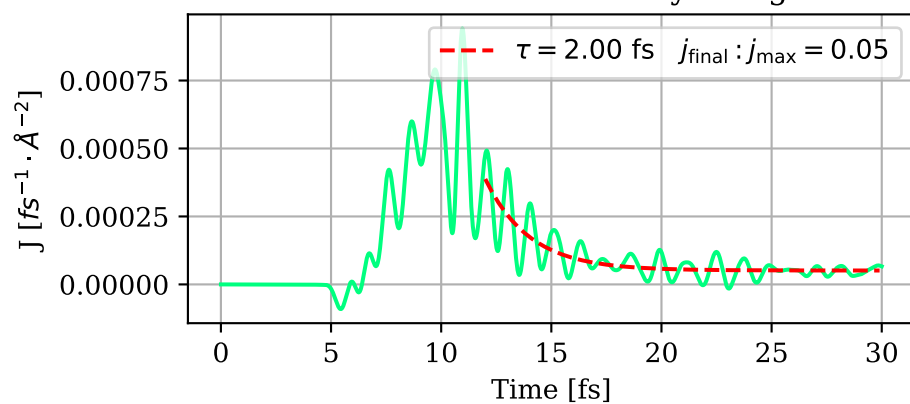
1e-5 \Delta matter current density along y
