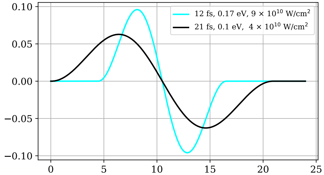
Probe electric field along the x-axis
