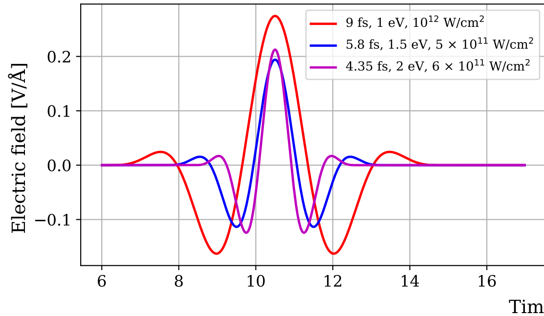
Pump electric field along the z-axis
