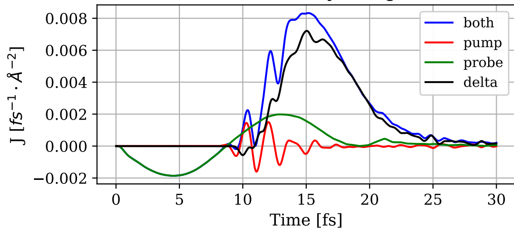
Matter current density along the x-axis
