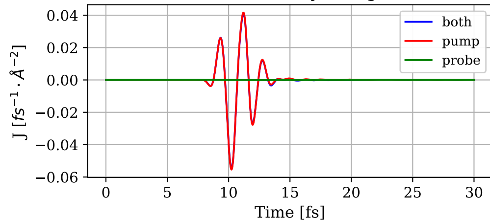
Matter current density along the z-axis
