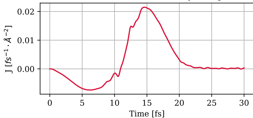
Full matter current density along y
