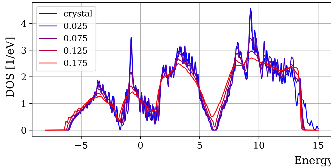
Displacement disorder
