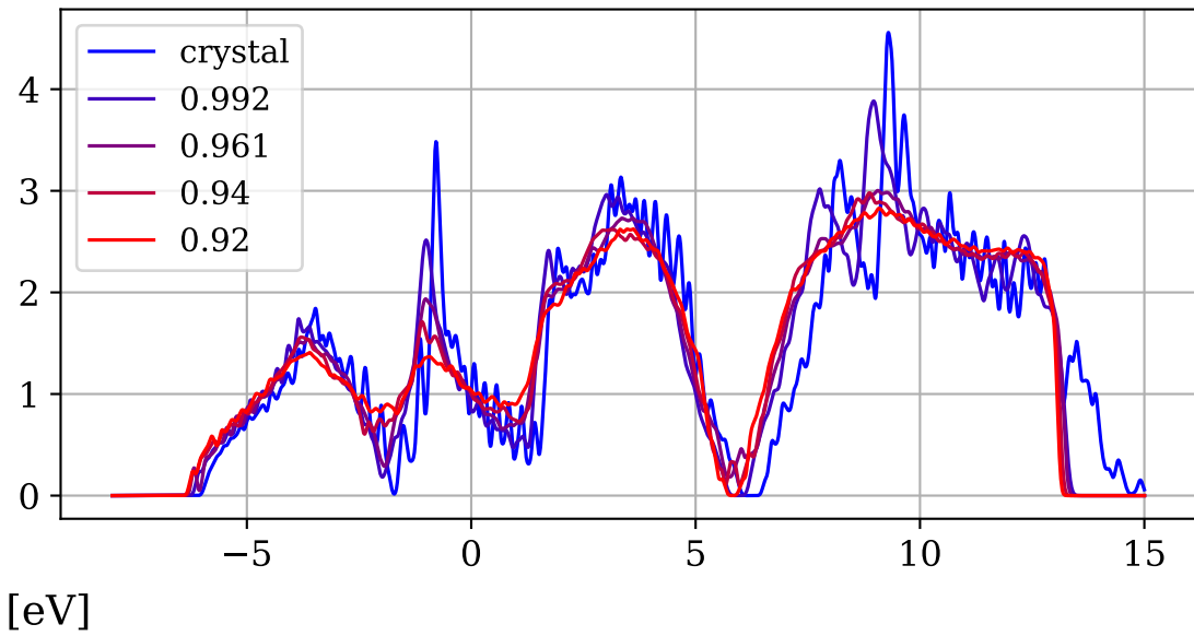
Amorphous disorder
