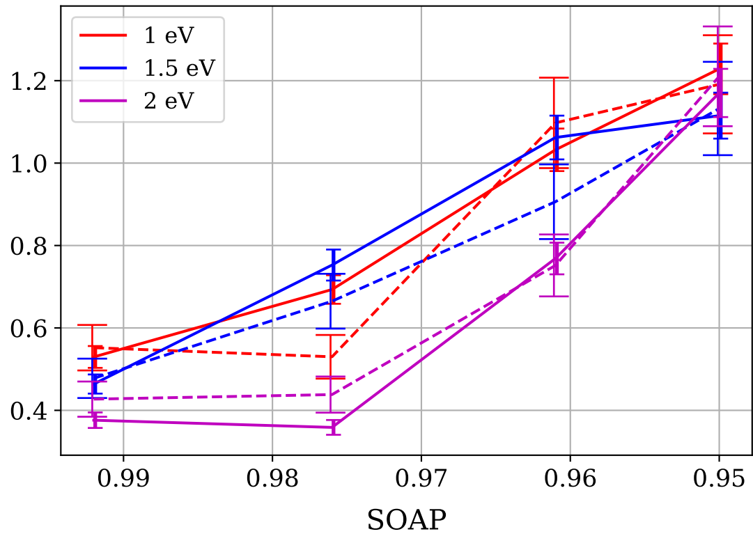
Amorphous disorder
