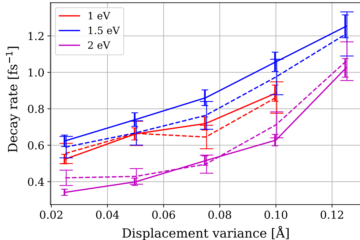
Displacement disorder
