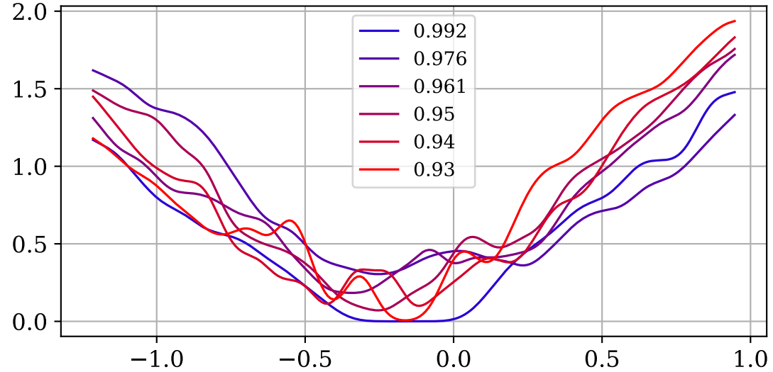
Amorphous disorder
