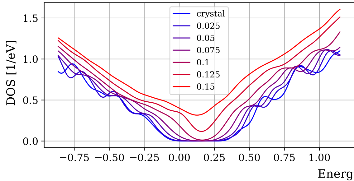
Displacement disorder
