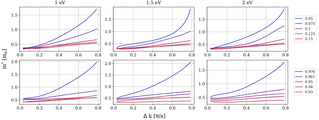
Figure 6.8: Crystal-momentum dependence of the effective mass. The column caption in eV indicates the carrier frequency of the pump pulse. The top row represents displacement disorder, whereas the bottom row represents amorphous disorder.
