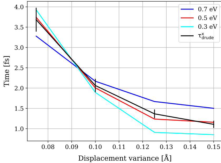
Figure 6.7: Urbach and relaxation time comparison.
