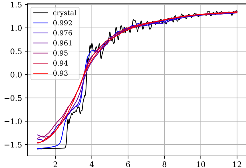
Amorphous disorder
