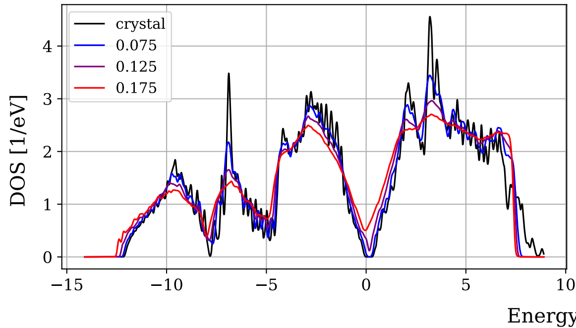
Displacement disorder
