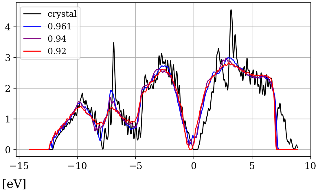
Amorphous disorder
