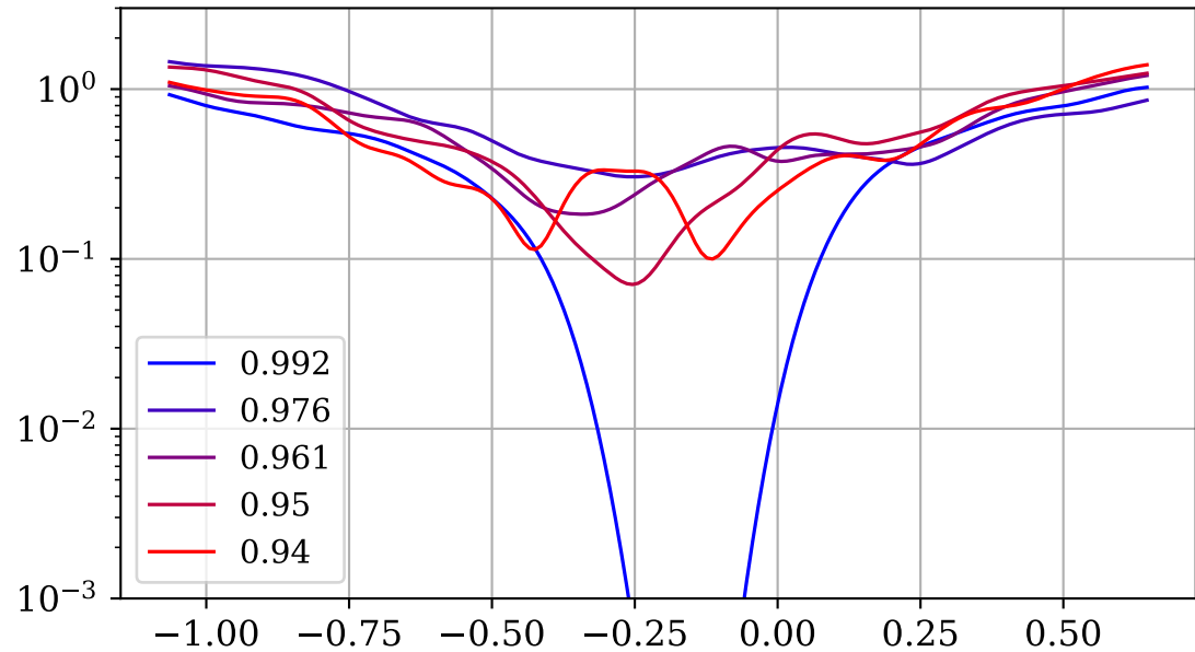
Amorphous disorder
