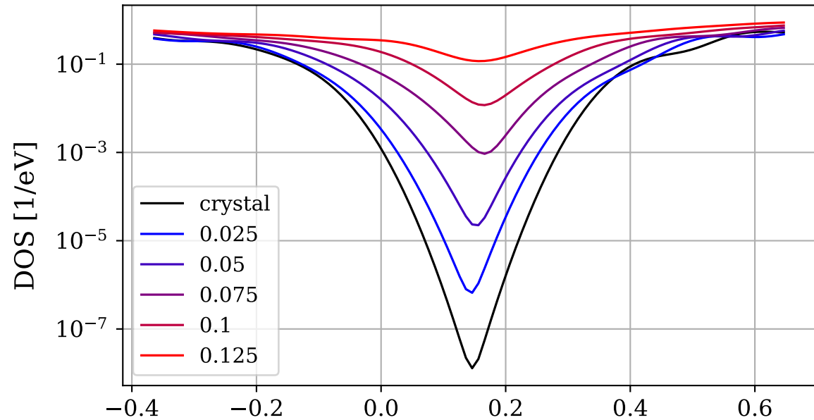
Displacement disorder
