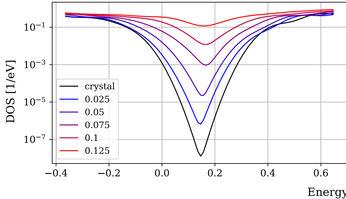
Displacement disorder
