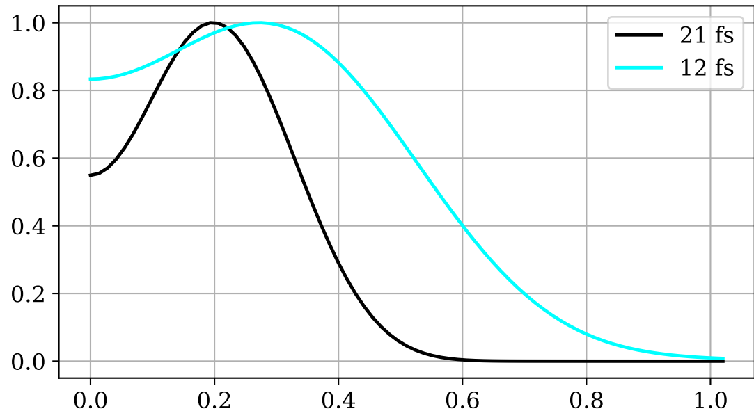
Probe electric field along the x-axis
