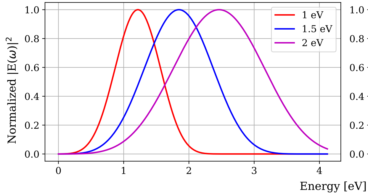
Pump electric field along the z-axis
