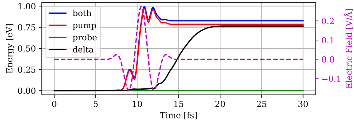
Energy transfer along z-direction
