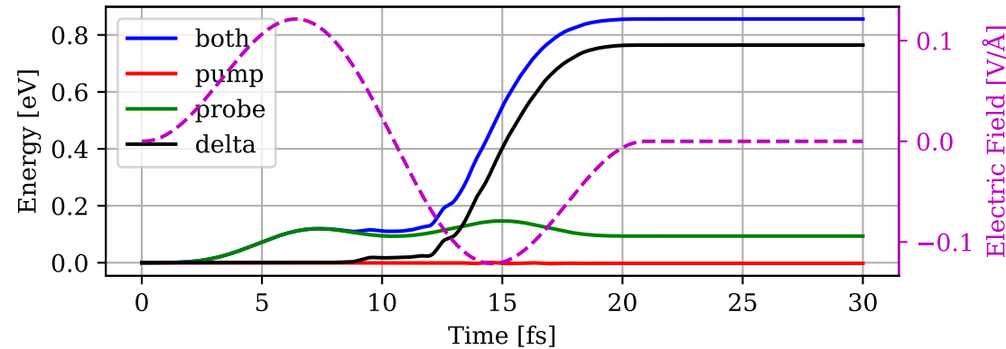
Energy transfer along x-direction
