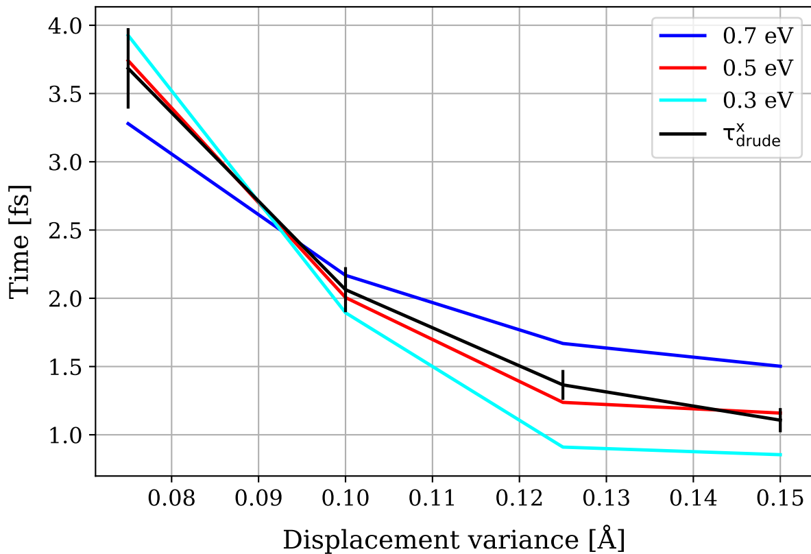
Comparison between \tau_{\text{drude}}^x and inverse E_U
