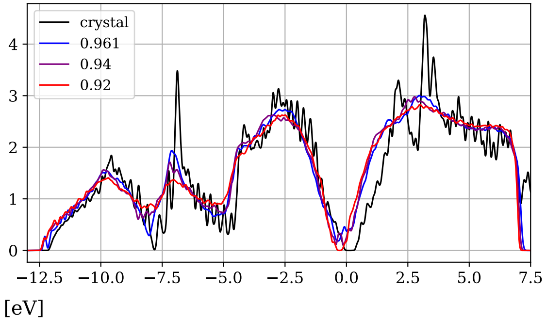
Amorphous disorder
