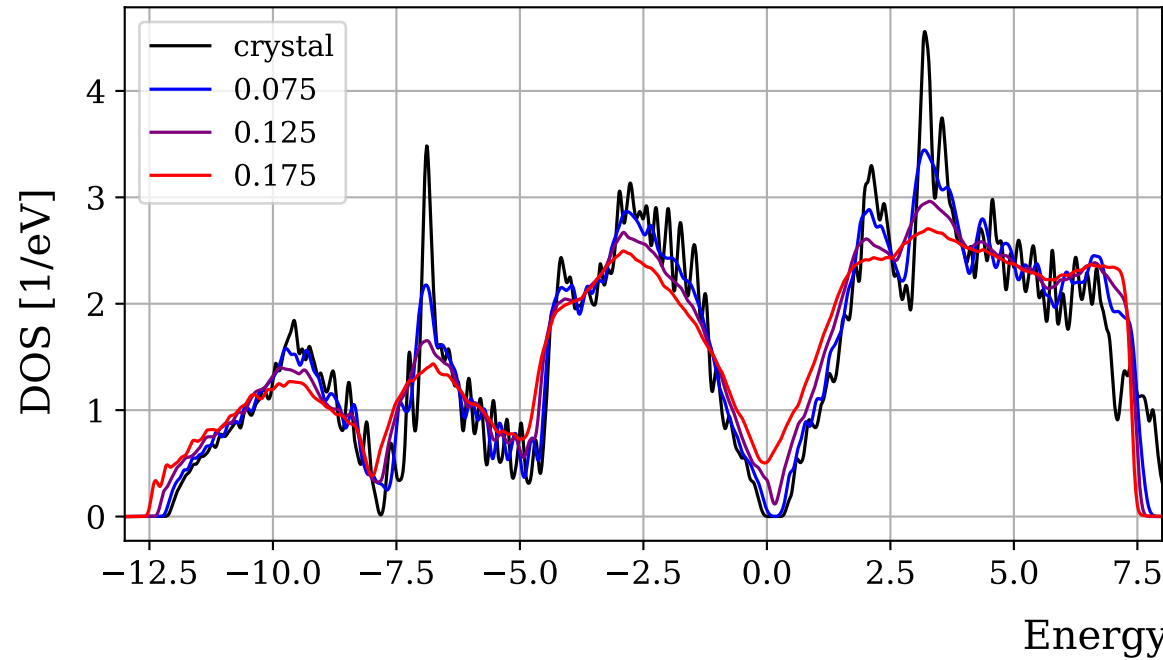
Displacement disorder
