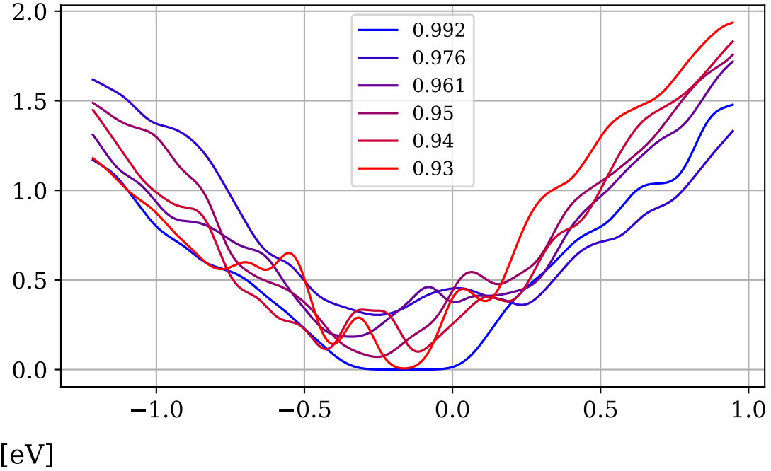
Amorphous disorder
