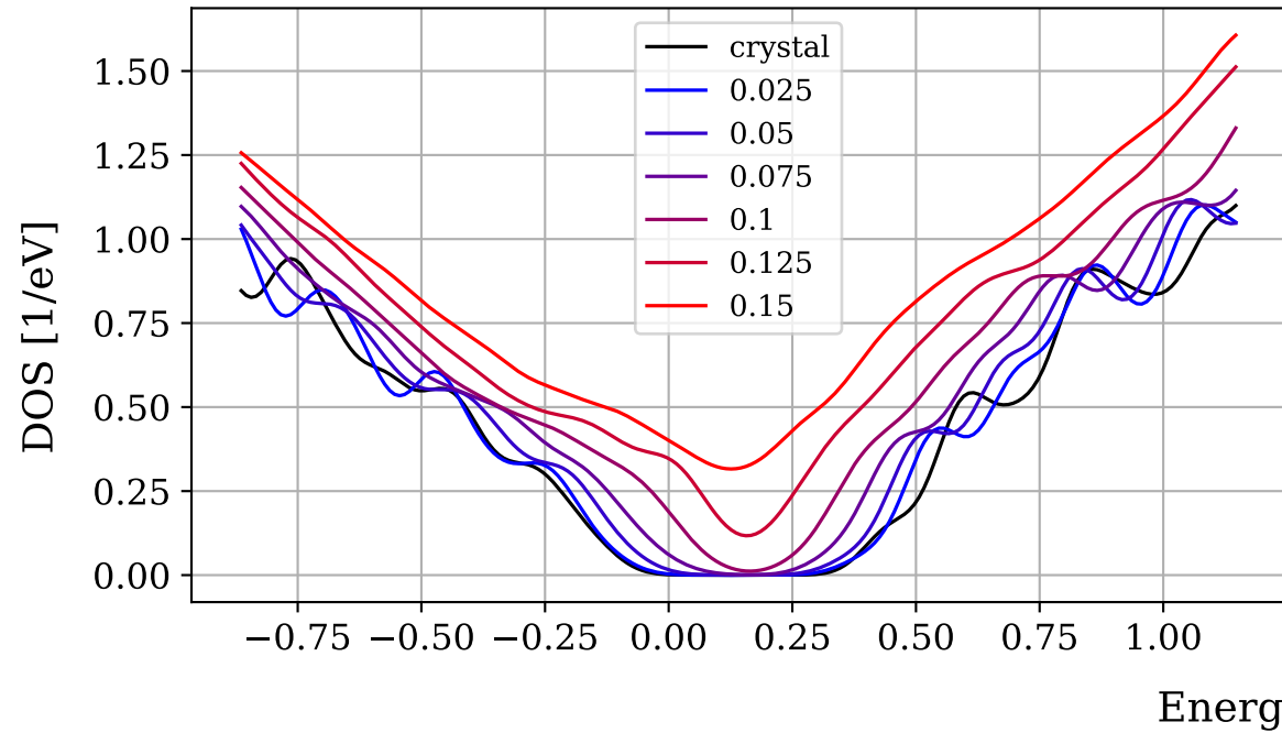
Displacement disorder
