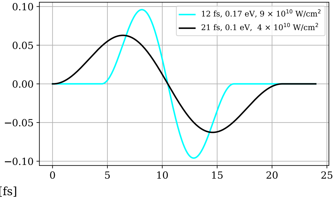
Probe electric field along the x-axis
