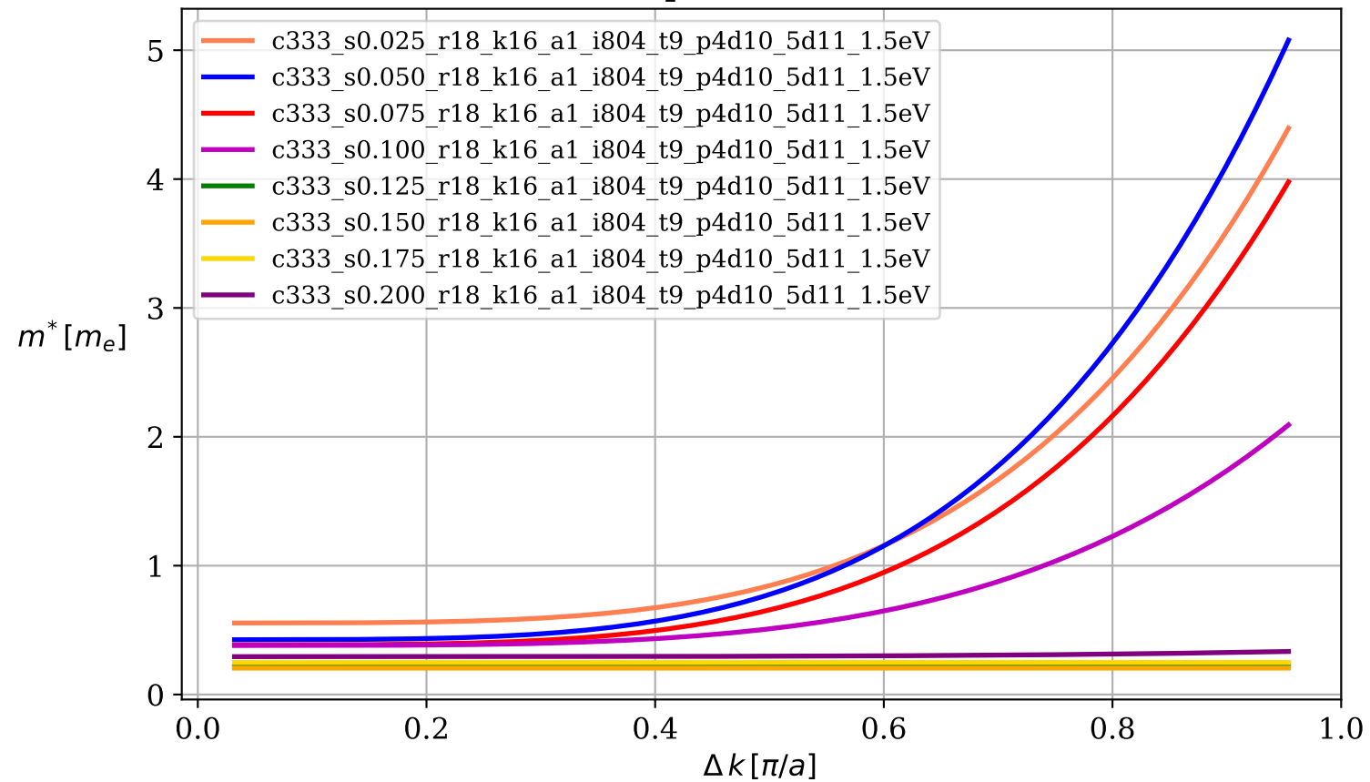
Drude mass dependence on wave vector
