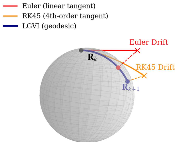
Figure 1. Position Update Mapping for Three Integration Methods Represented on the S^3 Manifold
