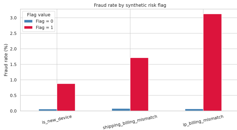
Figure 2: Fraud rate conditioned on each binary risk flag. When a flag is raised the fraud rate jumps by one to two orders of magnitude. The separation is striking—but it was designed into the generator (Section 3.5), which is precisely why these features are isolated in the Full feature space rather than mixed into Base.
