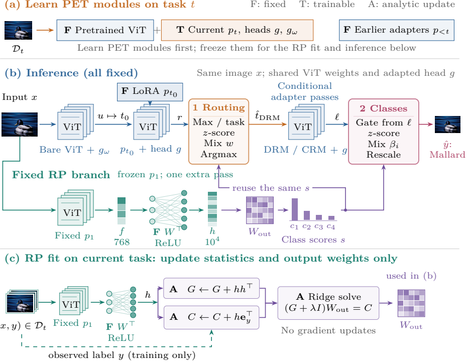
Fig. 1. Parameter lifecycle and two-stage fusion. (a) The inherited PET recipe trains adapters/heads, not the backbone. (b) All modules are fixed: Stage 1 revises the DRM proposal; Stage 2 gates class fusion using \ell . One RP score vector serves both stages. (c) Current training data update G, C, W_{\text{out}} analytically with fixed p_1, W . Only seen classes/tasks participate. Photos/bars are schematic, not measured predictions. Photo: T. G. Barnes/USFWS (public domain).
