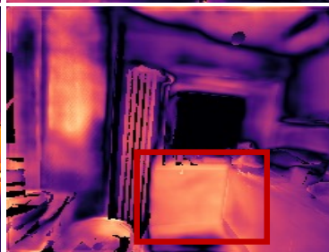
Mismatch (MASt3R)
