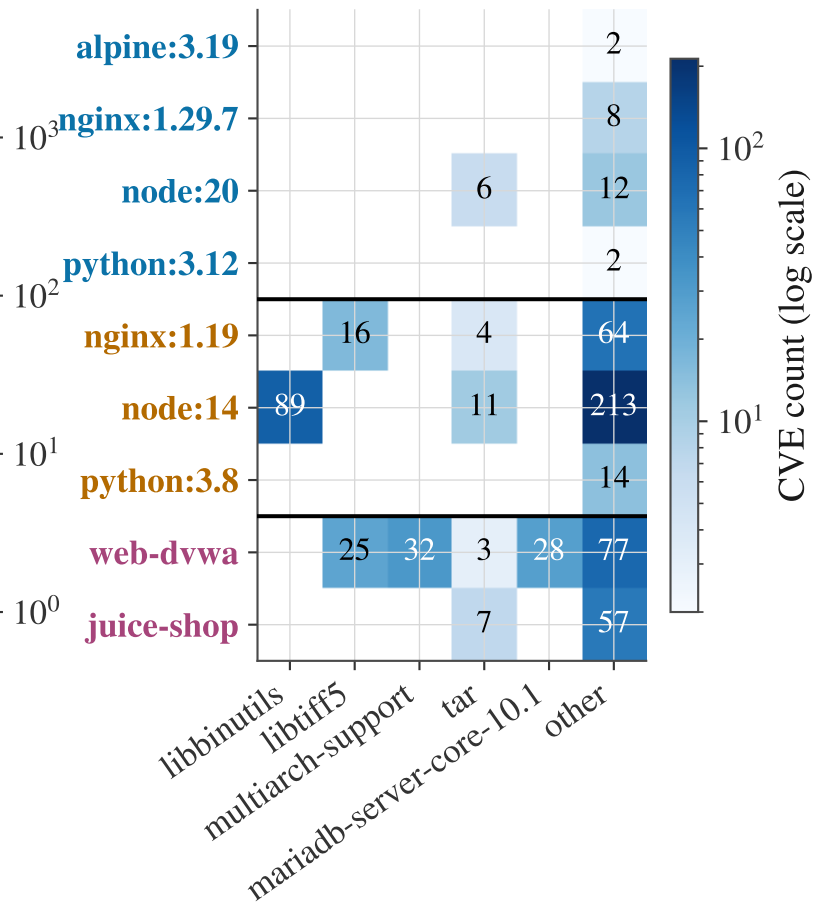
Grype-exclusive CVEs (G-only) by source package
