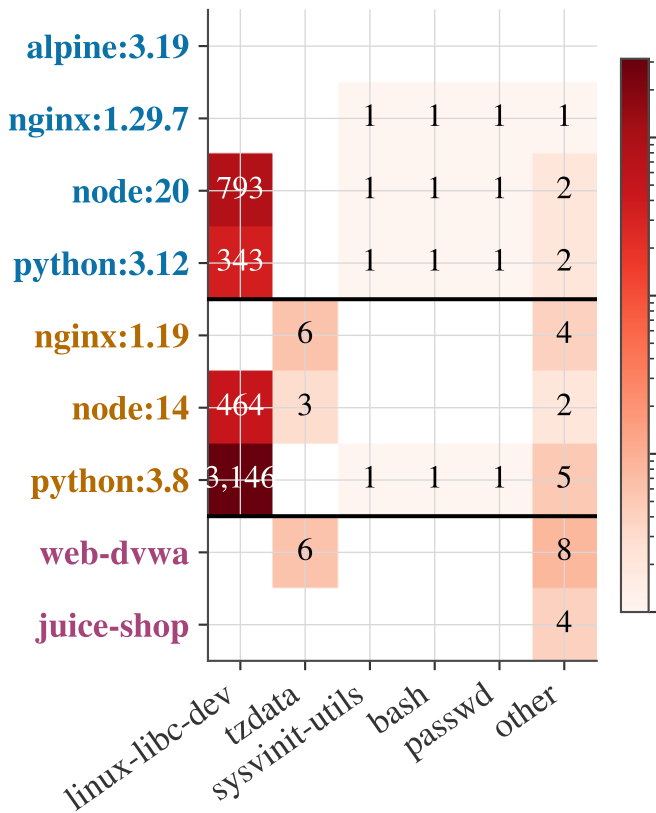
Trivy-exclusive CVEs (T-only) by source package
