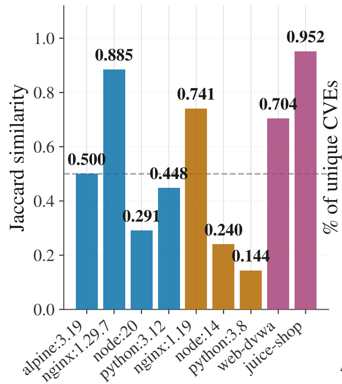
■ Group A ■ Group B ■ Group C ■ Shared (both) ■ Trivy only ■ Gype only (a) Jaccard similarity (b) CVE set composition
