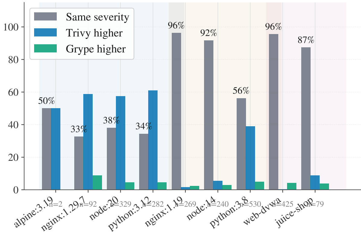
% of shared CVEs
