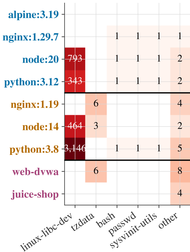
Fig 10 — Source Packages Driving CVE-Self Divergence (Trivy vs Gype) Trivy-exclusive CVEs (T-only) by source package Gype-exclusive CVEs (G-only) by source package
