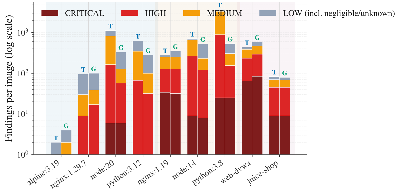
Fig 2 — Findings by Severity per Image (T=Trivy, G=Grype)
