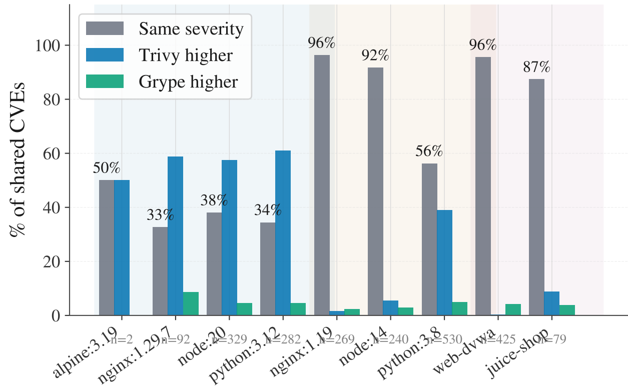
Fig 4 — Severity Agreement on Shared CVEs
