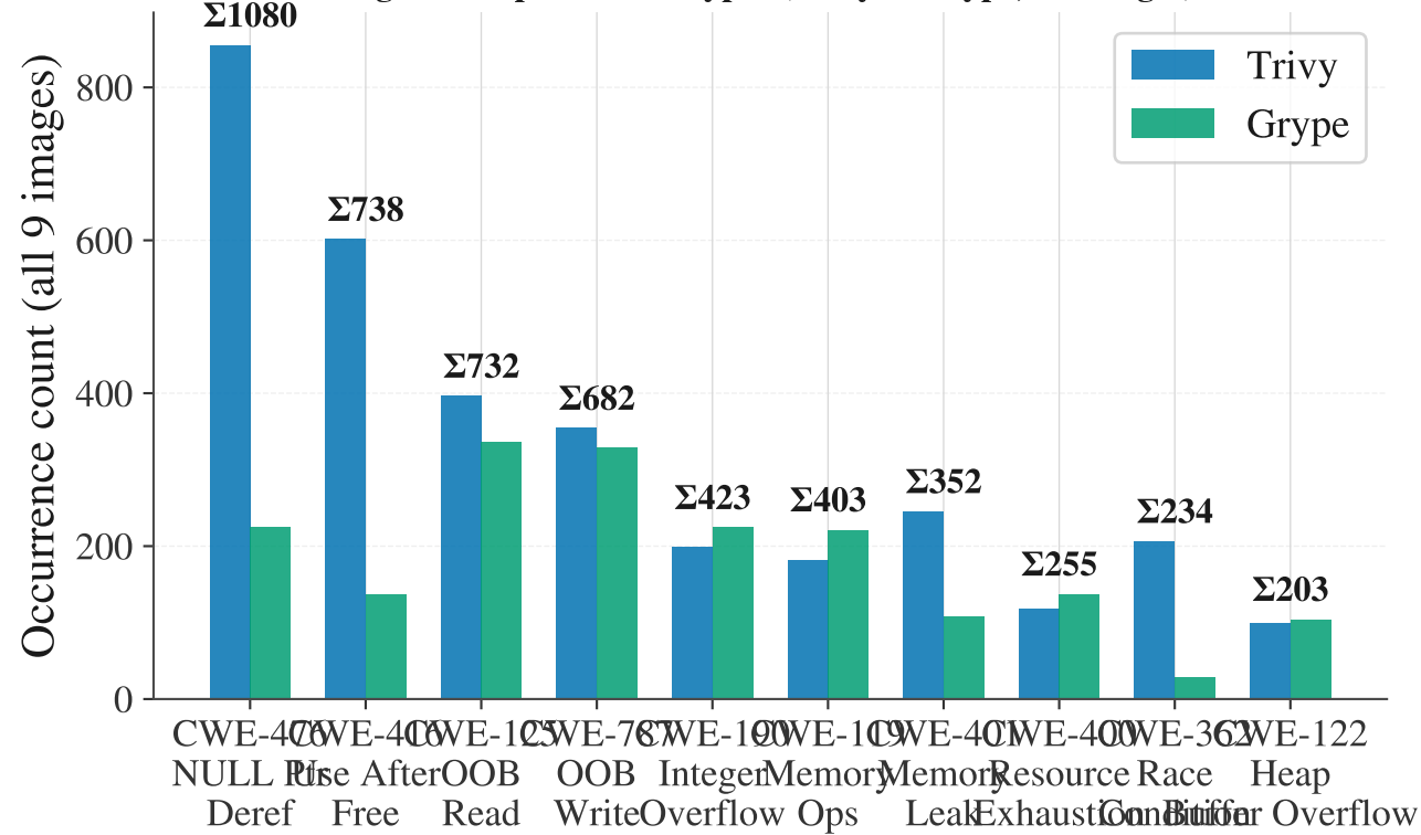
Fig 7 — Top 10 CWE Types (Trivy + Grype, all images)
