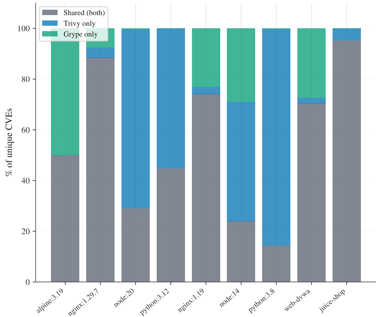
CVE Set Composition (Shared / Trivy-only / Gripe-only)
