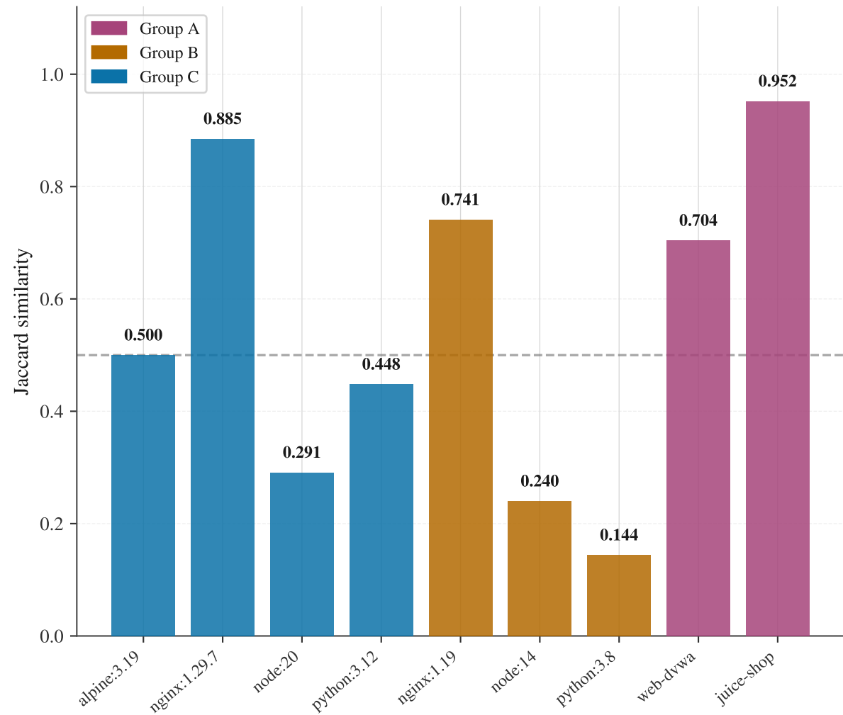
CVE-Level Overlap (Jaccard = |T \cap G| / |T \cup G| )
