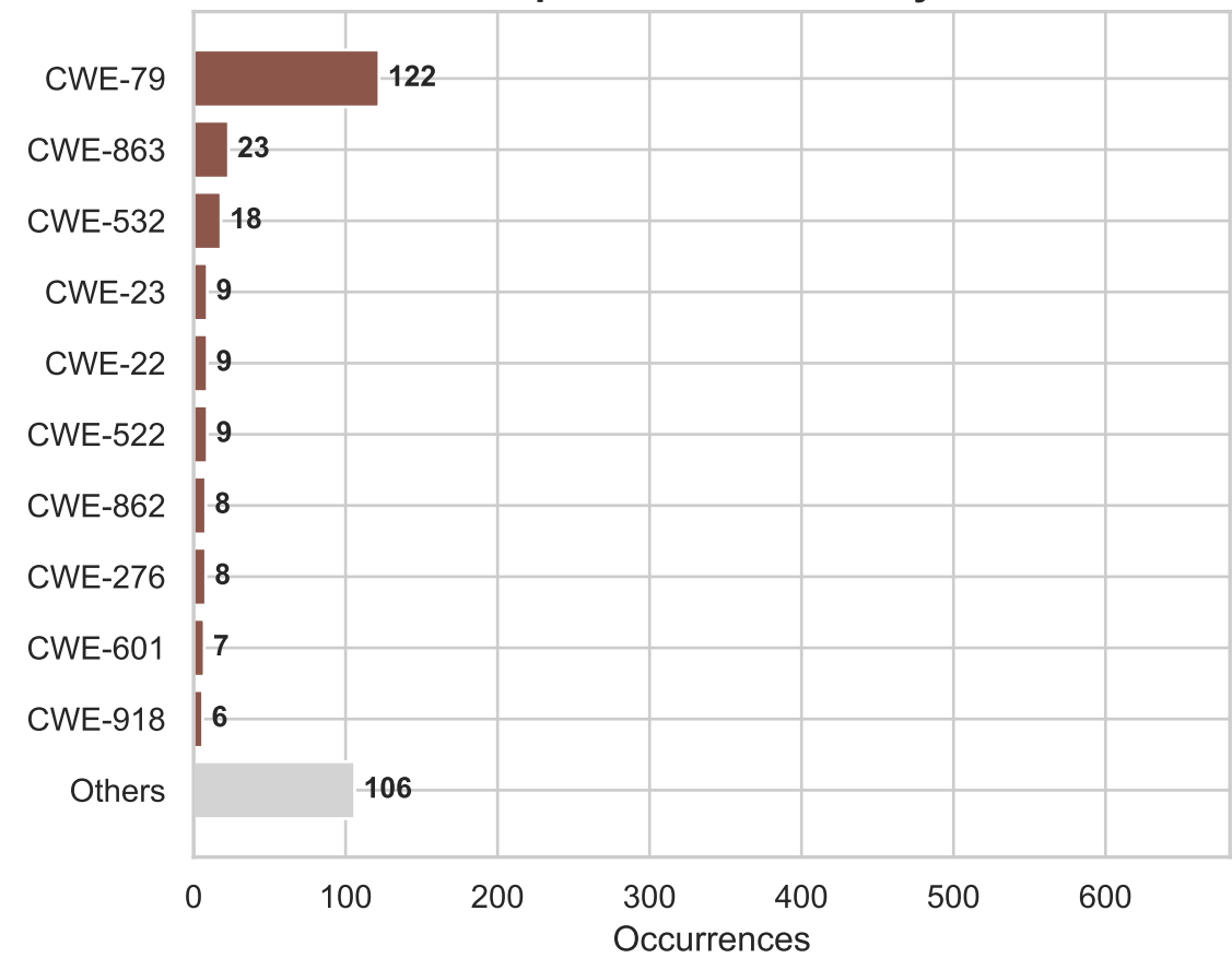
Top 10 CWEs: teamcity
