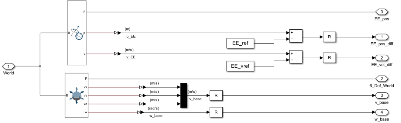
FIGURE 4: Overview of the Reference Subsystem in the Simulink Model SpaceRobot.slx
