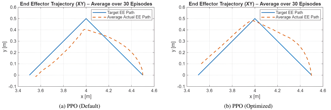
FIGURE 17: Target/actual comparison of the piecewise-linear end-effector trajectory in the XY plane.
