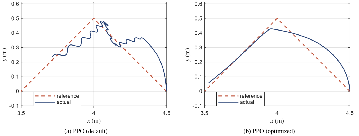
FIGURE 18: [R2.3] Reference and actual end-effector path on the piecewise-linear reference for one evaluation episode from the nominal initial state. The panels show the only successful run of the default PPO agent (seed 9) and the run of the optimized PPO agent with the median K_2 (seed 5).
