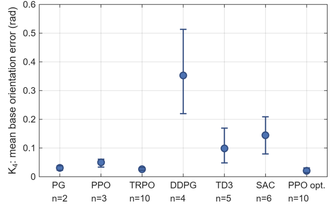
(b) K_4 : Mean Base Orientation Error
