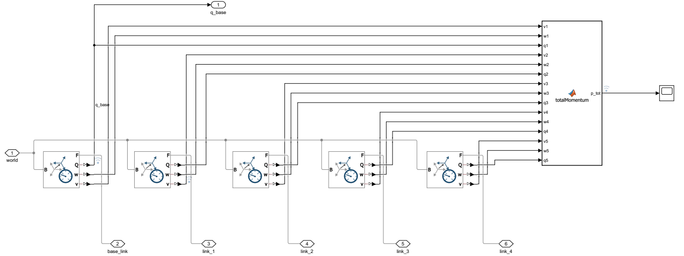
FIGURE 6: Momentum monitor subsystem (momentum observer) of the Simulink model SpaceRobot.slx . The velocities and orientations of the base and of all manipulator links are measured and combined in a MATLAB function to compute the total linear momentum of the free-floating space robot. The monitor is used to check momentum conservation in the simulation.
