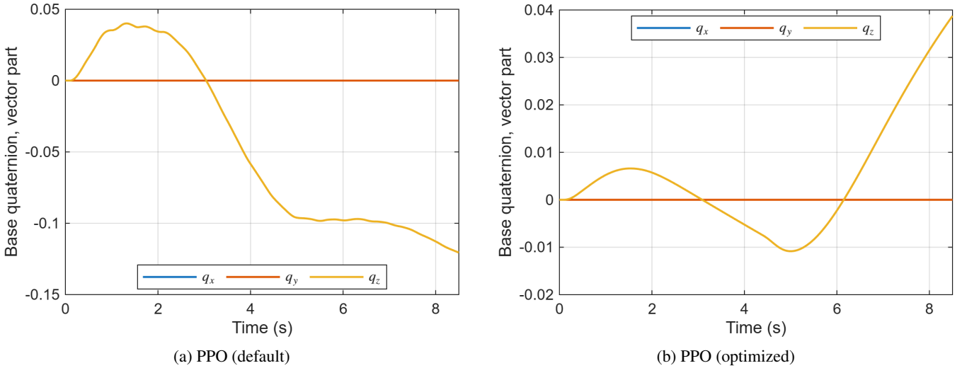
FIGURE 19: [R2.3] Vector part of the base orientation quaternion during the episodes of Fig. 18. The base rotates only about the z -axis. The scalar part stays above 0.992 for the default and above 0.999 for the optimized agent.
