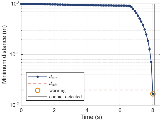
(a) Minimum distance between non-adjacent bodies
