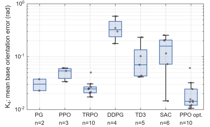
(b) K_4 : Mean Base Orientation Error
