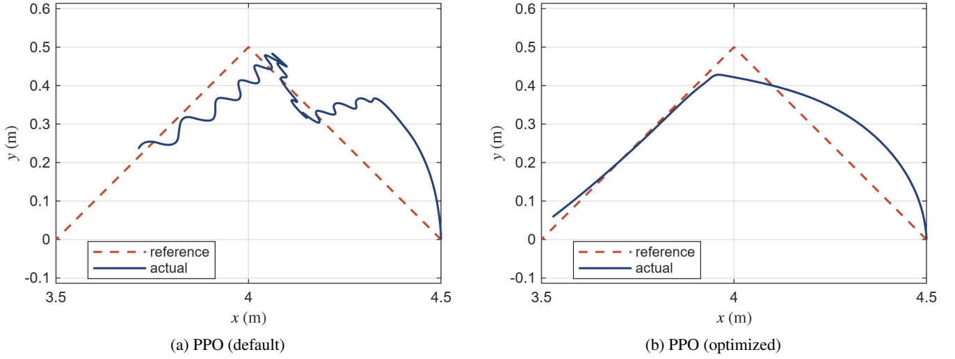
FIGURE 18: Reference and actual end-effector path on the piecewise-linear reference for one evaluation episode from the nominal initial state. The panels show the only successful run of the default PPO agent (seed 9) and the run of the optimized PPO agent with the median K_2 (seed 5).
