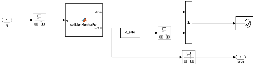
FIGURE 8: Collision monitor subsystem of the Simulink model SpaceRobot.slx . [A60] The joint angles q are used to compute the minimum distance between non-adjacent robot bodies. A distance below the safety threshold d_{\text{safe}} triggers the assertion block, which raises a warning. A detected contact sets the collision flag, which terminates the episode.
