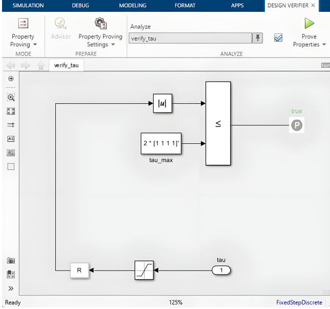
FIGURE 10: [A45] Verification model for Simulink Design Verifier (verify_tau.slx). The torque command \tau is an unconstrained input and passes through a saturation block with the limits \pm\tau_{\max} . A relational operator compares the absolute saturated torques with \tau_{\max} = 2 \text{ N m} , and a proof objective (P) requires this comparison to be true.
