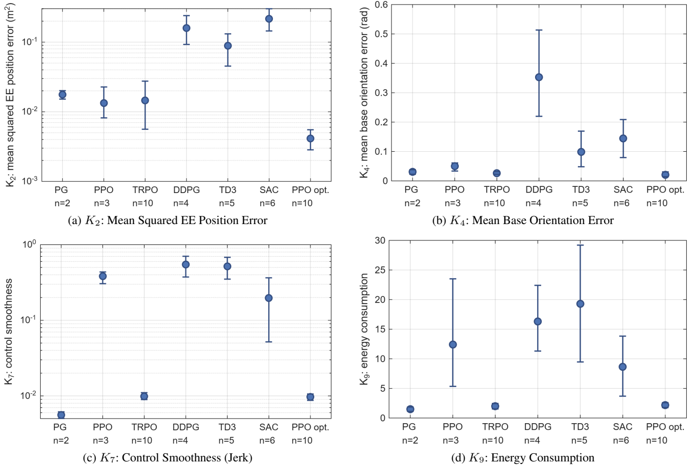
FIGURE 14: [R2.3, A9] Mean and 95% bootstrap confidence interval of selected KPIs over the successful runs of each agent (2000 resamples). The number of successful runs is given below each agent. The intervals of agents with few successful runs are wide or undefined. The optimized PPO agent of Section VII is included for reference.
