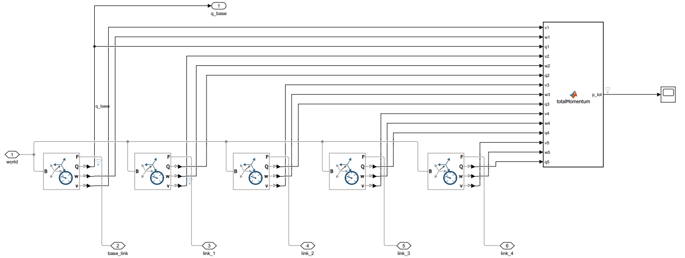
FIGURE 6: Momentum monitor subsystem (momentum observer) of the Simulink model SpaceRobot.slx . [A27] The velocities and orientations of the base and of all manipulator links are measured and combined in a MATLAB function to compute the total linear momentum of the free-floating space robot. The monitor is used to check momentum conservation in the simulation.
