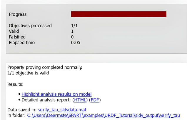
FIGURE 11: Result of Simulink Design Verifier for the torque-bound property. [R2.1, A45] The proof objective of Fig. 10 is valid for any value of the input \tau , and no counterexample was found. The result covers only the saturation of the actuation path, not the policy network, the plant, or other properties.
