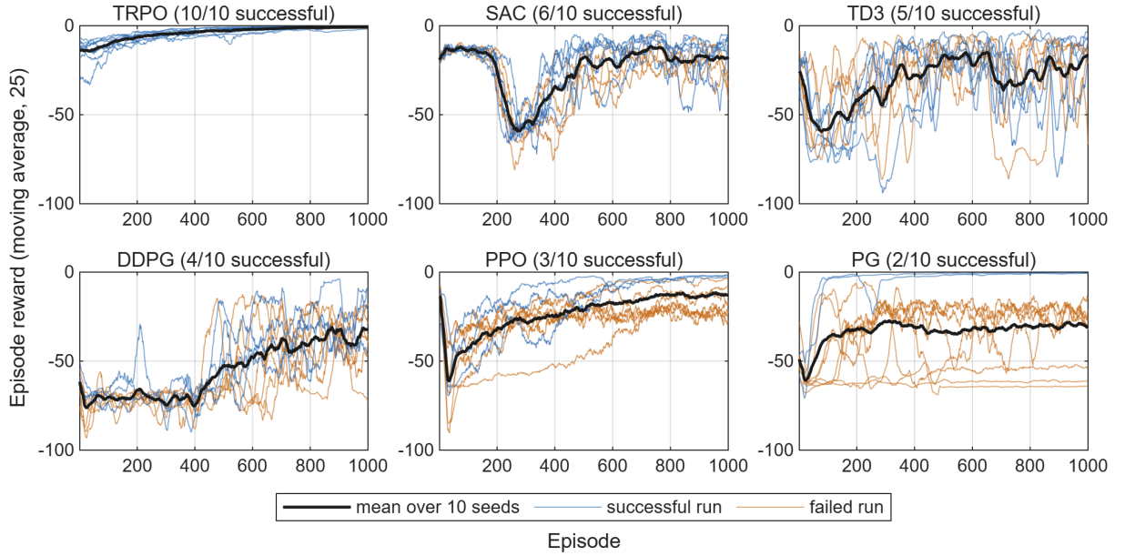
FIGURE 12: [A55] Episode rewards during training of the six default agents over ten seeds each. Each thin line shows one seed as a moving average over 25 episodes. Blue lines are successful runs, orange lines are failed runs, and the black line is the mean over the ten seeds. All panels use the same axis.
