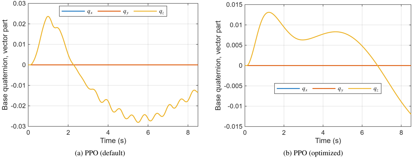
FIGURE 17: [R2.3, A9] Vector part of the base orientation quaternion during the episodes of Fig. 16. The base rotates only about the z -axis. The scalar part stays above 0.9996 in both episodes.
