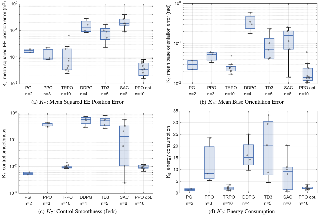
FIGURE 13: [R2.3, A9] Distribution of selected KPIs over the successful runs of each agent. Each point is one run, averaged over the 30 random initial states, and the number of successful runs is given below each agent. Each box spans the interquartile range, and the center line marks the median. Axes are logarithmic where the values span more than a factor of 50. The optimized PPO agent of Section VII is included for reference.
