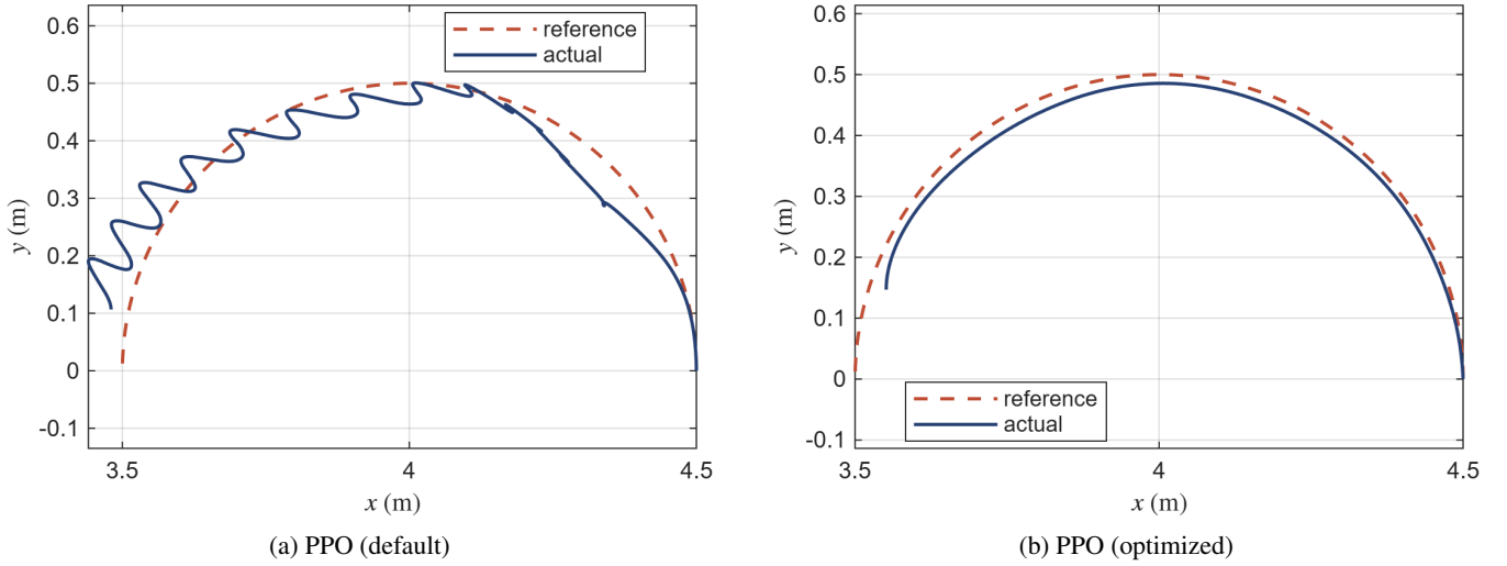
FIGURE 16: [R2.3, A9] Reference and actual end-effector path in the XY plane for one evaluation episode from the nominal initial state. Each panel shows the successful run with the median K_2 of its configuration, seed 2 for the default and seed 0 for the optimized PPO agent.
