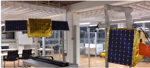
FIGURE 16: Our testbed for In-Space Robotized Services.
