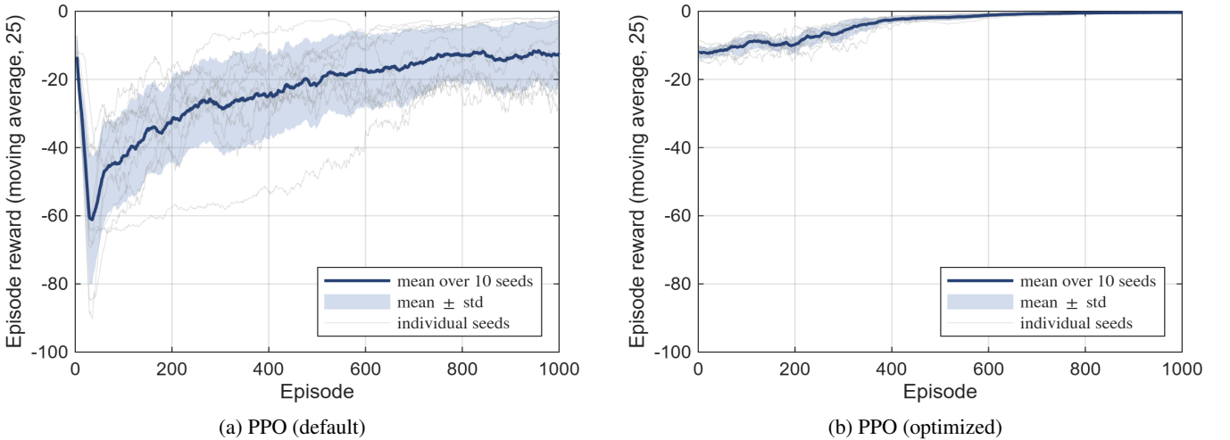
FIGURE 15: Episode rewards during training of the default and the optimized PPO agents over ten seeds. The thin lines show the moving average over 25 episodes of each seed, the thick line the mean over the seeds, and the band one standard deviation. Both panels use the same axis. (a) Default hyperparameters. (b) Optimized configuration.
