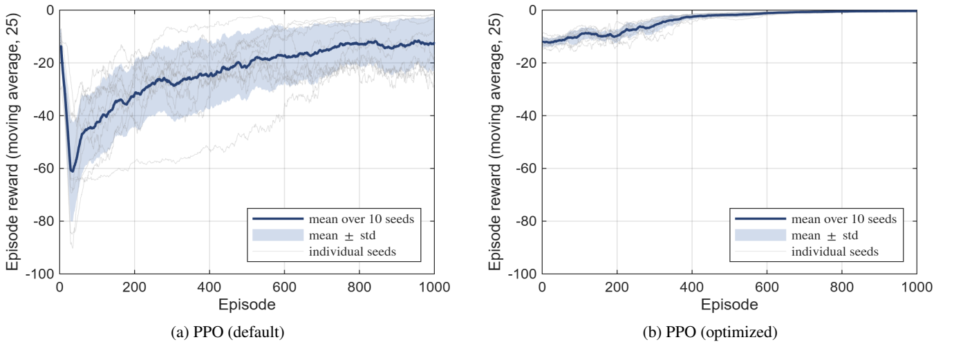
FIGURE 15: [R2.3] Episode rewards during training of the default and the optimized PPO agents over ten seeds. The thin lines show the moving average over 25 episodes of each seed, the thick line the mean over the seeds, and the band one standard deviation. Both panels use the same axis. (a) Default hyperparameters. (b) Optimized configuration.
