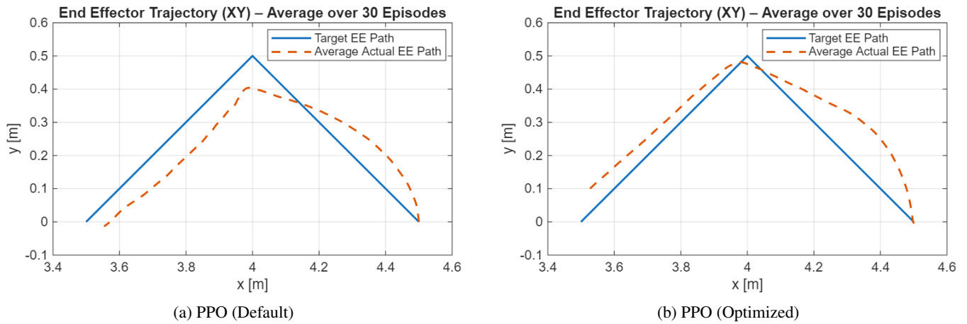
FIGURE 17: Target/actual comparison of the ramp end-effector trajectory in the XY plane.
