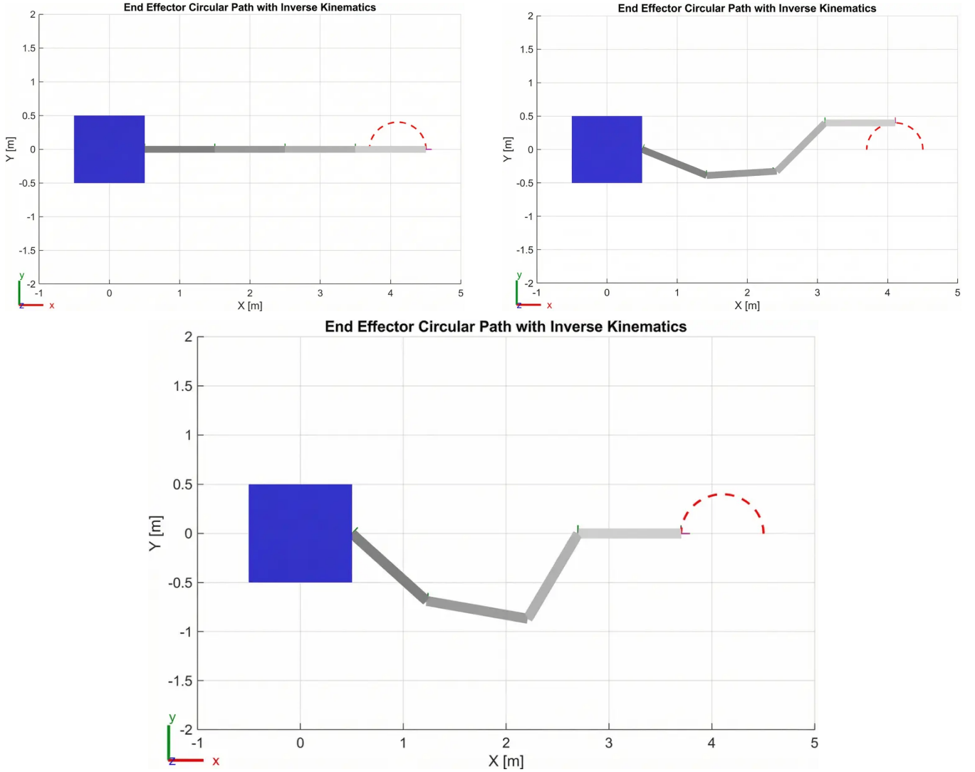
FIGURE 1: Tracking the desired end-effector circular path using inverse kinematics.
