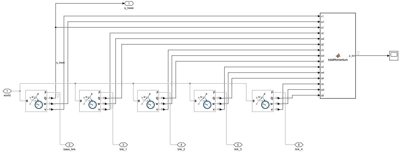
FIGURE 6: Momentum monitor subsystem (momentum observer) of the Simulink model SpaceRobot . slx . The velocities and orientations of the base and of all manipulator links are measured and combined in a MATLAB function to compute the total linear momentum of the free-floating space robot. The monitor is used to check momentum conservation in the simulation.
